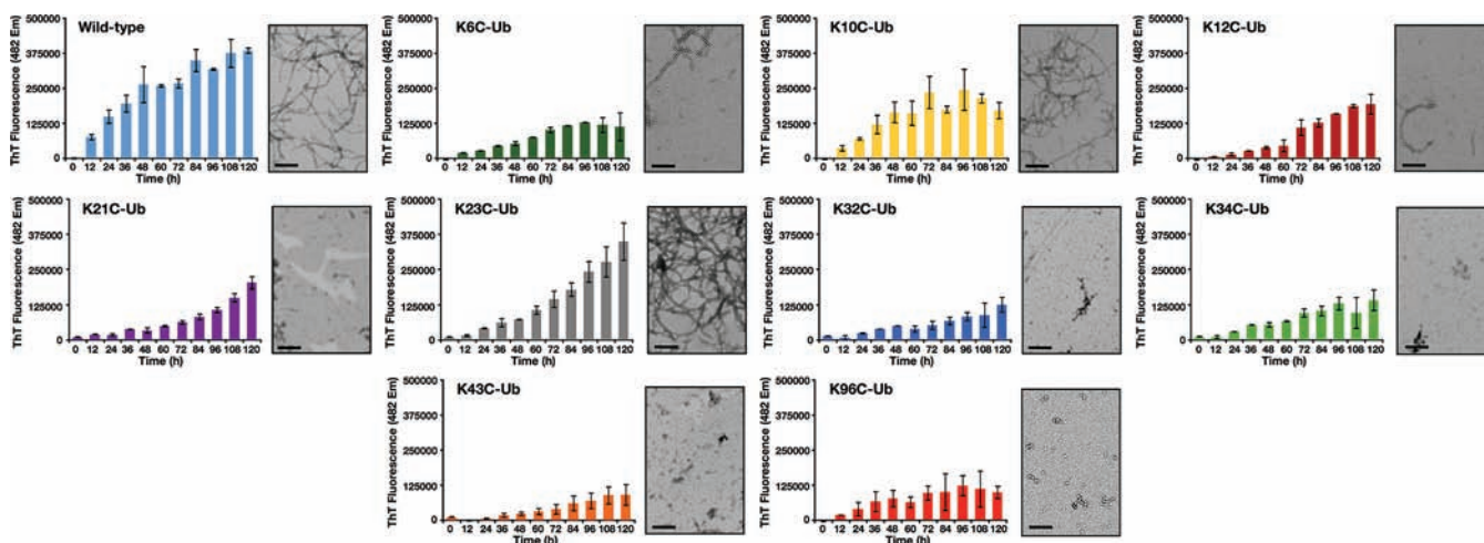
Figure 3. Aggregation of ubiquitinated \alpha -synuclein. Purified \alpha -synuclein ( \alpha -Syn) and the disulfide-directed ubiquitinated derivatives (K#C-Ub) at a concentration of 100 \mu\text{M} were incubated at 37^\circ\text{C} before analysis by ThT fluorescence ( 450 \text{ nm Ex}/482 \text{ nm Em} ) at the indicated time points. The same protein samples at day 5 were analyzed by TEM; scale bar: 500 \text{ nm} . The experiments were performed in triplicate and error bars represent standard deviation.
