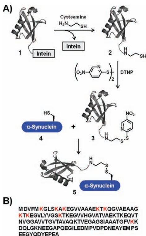
Figure 1. Disulfide-directed ubiquitination of \alpha -synuclein. (A) Ubiquitin was expressed in Escherichia coli as a fusion to the GyrA intein (1). Intein-mediated thiolysis with cysteamine yielded 2 and subsequent reaction with DTNP generated the activated ubiquitin mixed disulfide (3). \alpha -Synuclein cysteine point mutants (4) were also expressed in E. coli and were then reacted with 3 to generate the corresponding disulfide-directed ubiquitinated derivatives. (B) Primary sequence of \alpha -syn with all sites of ubiquitination noted in red.
